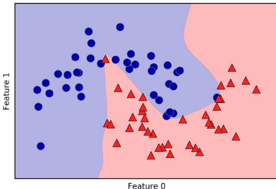
Figure 2-51. Decision boundary learned using 2 hidden layers with 10 hidden units each, with tanh activation function
